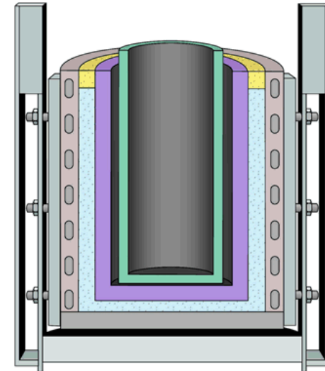
Section through a vacuum furnace
