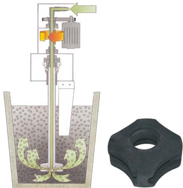
Figure 5: Effective degassing process using a Foseco Degassing Unit (left) and the patented impeller rotor (right)
