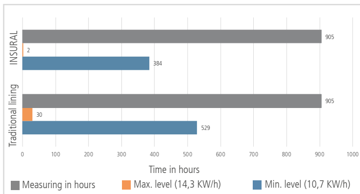
Diagram 3: Power consumption
