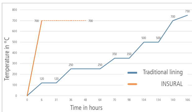
Diagram 1: Comparison of preheating curves
