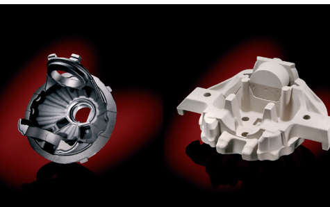
Rear axle housing and core subassembly
