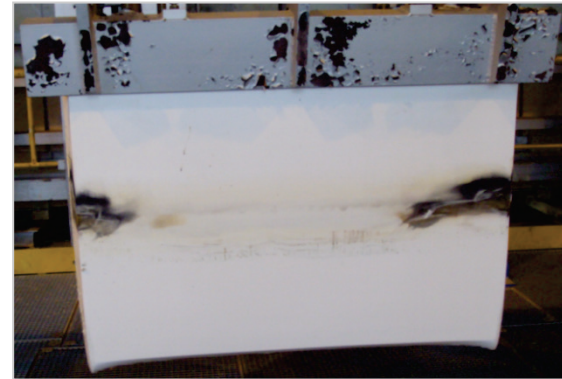
ZYAROCK® tweel after production of 425.000 tons of float glass for architectural market
