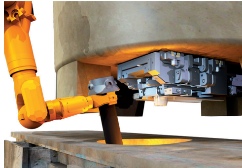
Robotized operation with ladle tube changer
