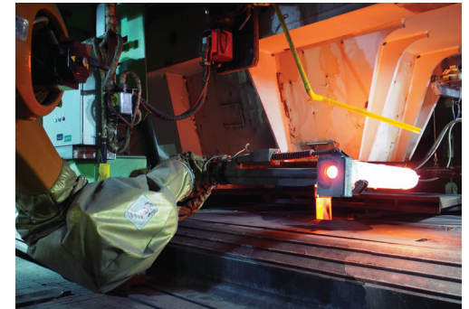
Fully automatic tube change for stopper or tundish slide gate
